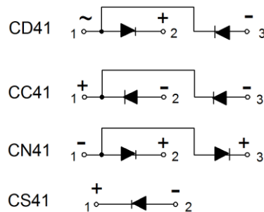
CONNECTION DIAGRAMS
