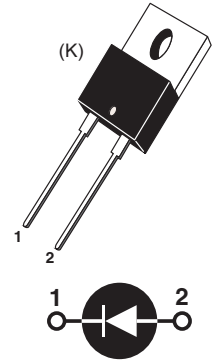
1 - Cathode 2 - Anode Back of Case - Cathode
