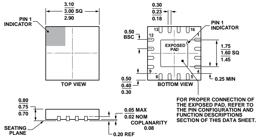
Figure 68. 16-Lead Lead Frame Chip Scale Package [LFCSP_WQ] 3 mm × 3 mm Body, Very Very Thin Quad (CP-16-22) Dimensions shown in millimeters
