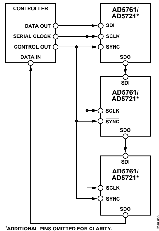
Figure 65. Daisy-Chain Block Diagram
