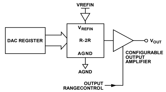
Figure 63. DAC Architecture
