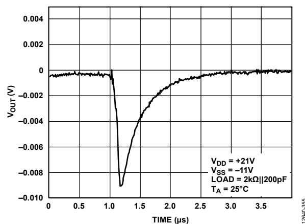
Figure 48. Digital-to-Analog Glitch Energy, \pm 10 V Range
