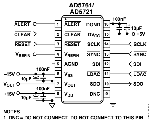
Figure 66. Typical Operating Circuit
