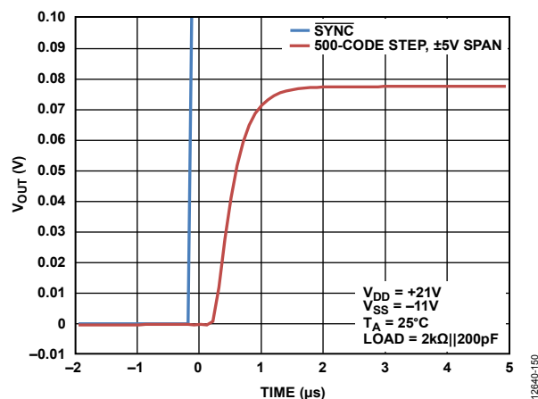
Figure 43. 500-Code Step Settling Time, \pm 5 V Range
