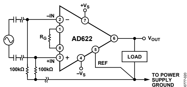
Figure 21. Ground Returns for Bias Currents with AC-Coupled Inputs
