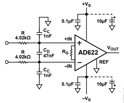
Figure 18. RFI Suppression Circuit for AD622 Series In-Amps
