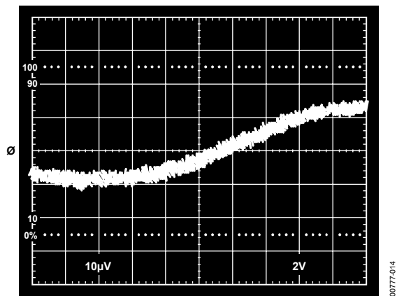
Figure 14. Gain Nonlinearity, G = 1 , R_L = 10 \text{ k}\Omega ( 20 \mu\text{V} = 2 \text{ ppm} )
