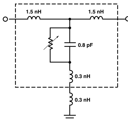
Figure 16. Equivalent Circuit.
