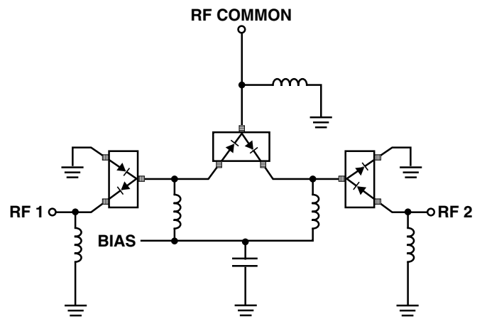
Figure 10. Very High Isolation SPDT Switch, Dual Bias.
