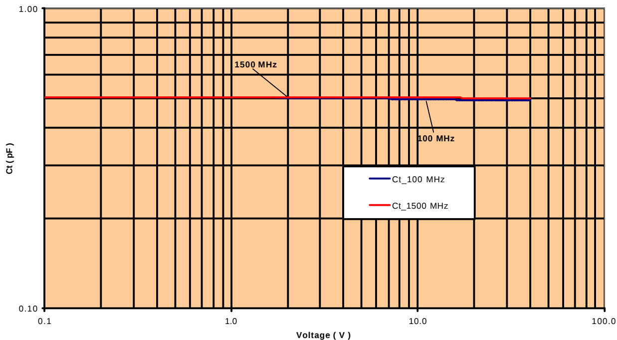
MA4P7452F-1072T Ct vs Voltage
