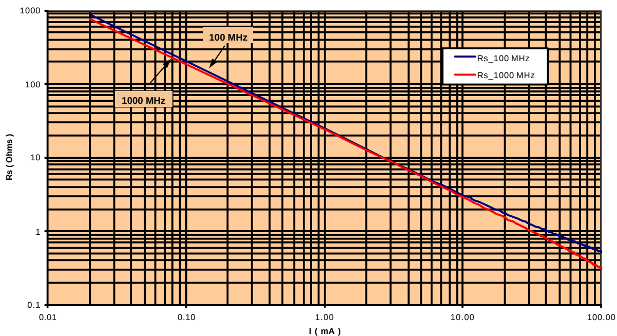
MA4P7452F-1072T R_s vs I
