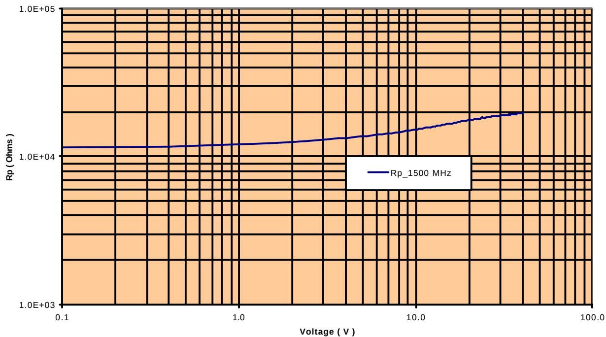
MA4P7452F-1072T R_p vs Voltage
