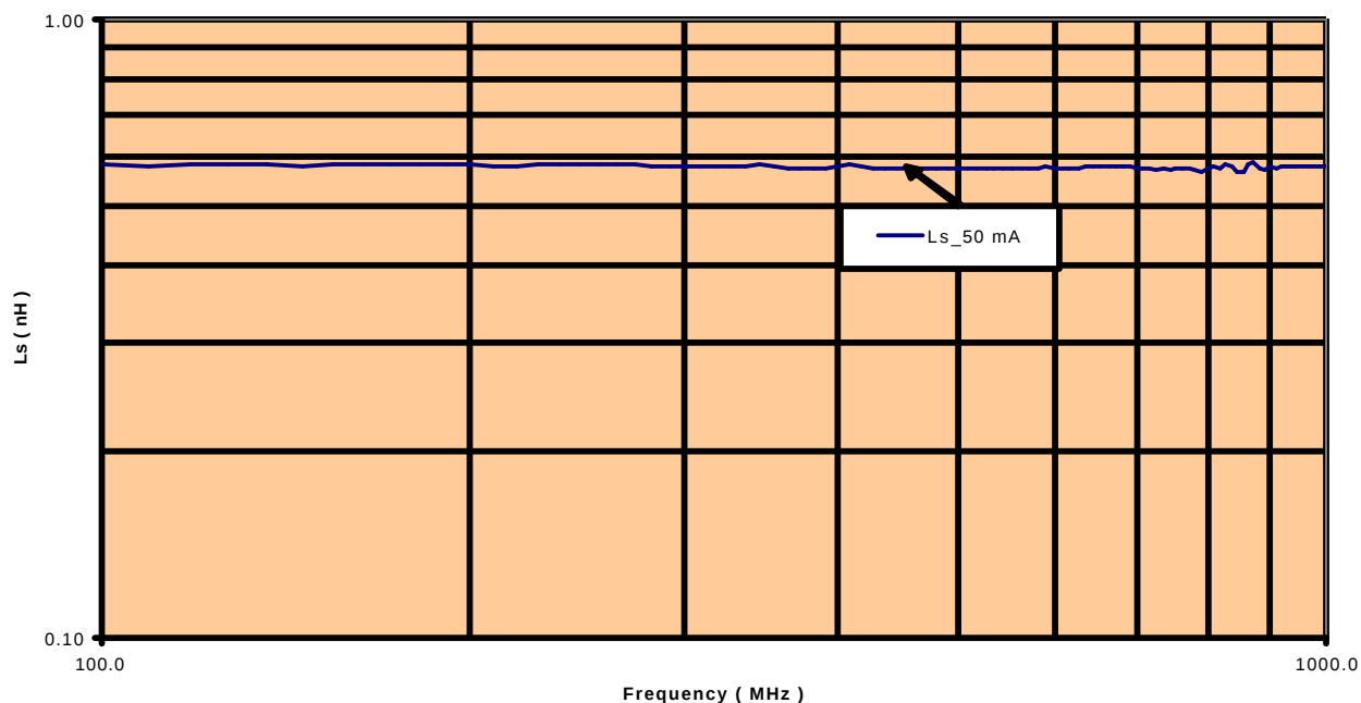
MA4P7452F-1072T Ls vs Frequency
