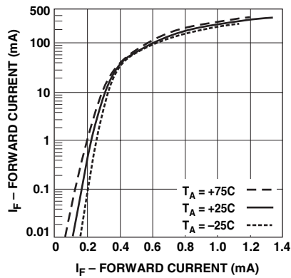
Figure 2. Forward Current vs. Forward Voltage at Temperature for HBA5-540B and HBA5-540C.
