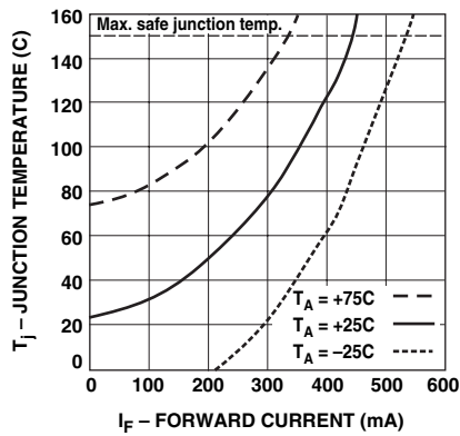
Figure 4. Junction Temperature vs. Current as a Function of Heat Sink Temperature for HBA5-540B and HBA5-540C.
