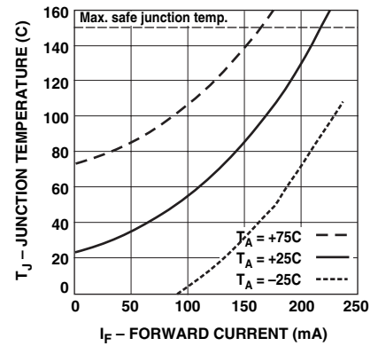
Figure 3. Junction Temperature vs. Current as a Function of Heat Sink Temperature for HBA5-5400 and HBA5-5402.
