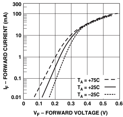
Figure 1. Forward Current vs. Forward Voltage at Temperature for HBA5-5400 and HBA5-5402.
