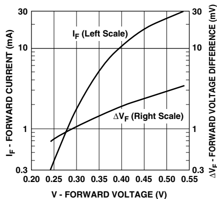
Figure 2. Typical VF Match, HSMS-820X Pairs and Ouads.
