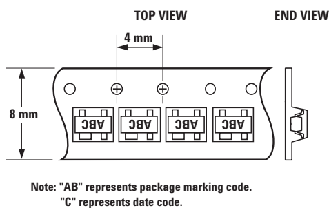
Figure 5. Option -TR1G/-TR2G for SOT-143 Packages.
