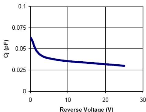
Typical Capacitance vs. Reverse Bias Voltage
