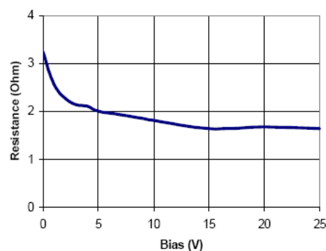
Typical Resistance vs. Reverse Bias Voltage
