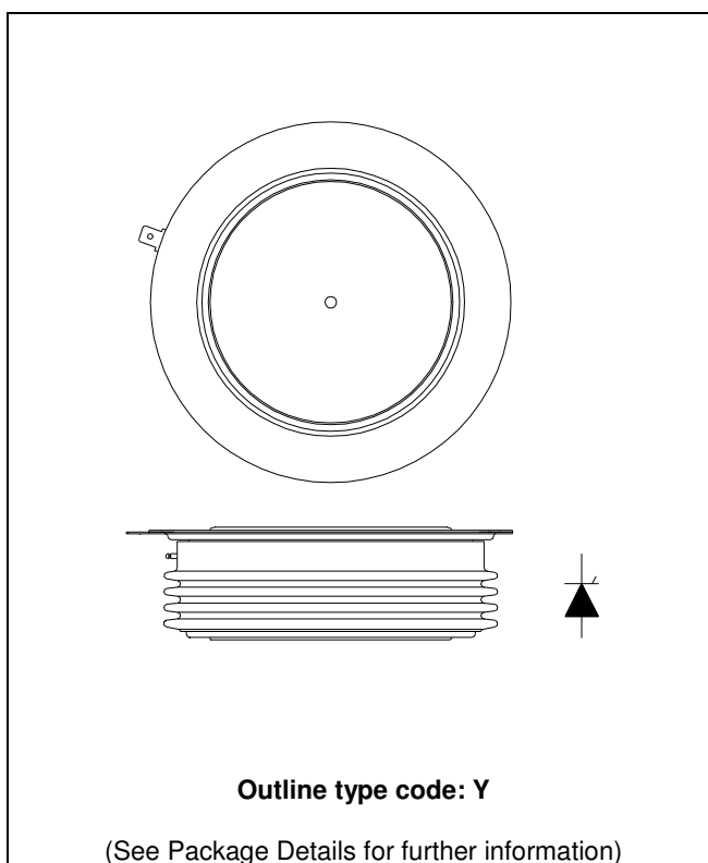
Fig. 1 Package outline
