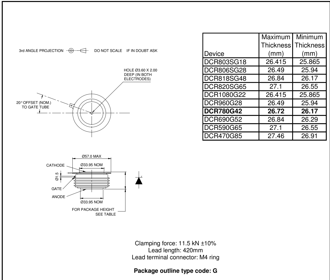
Fig.14 Package outline
