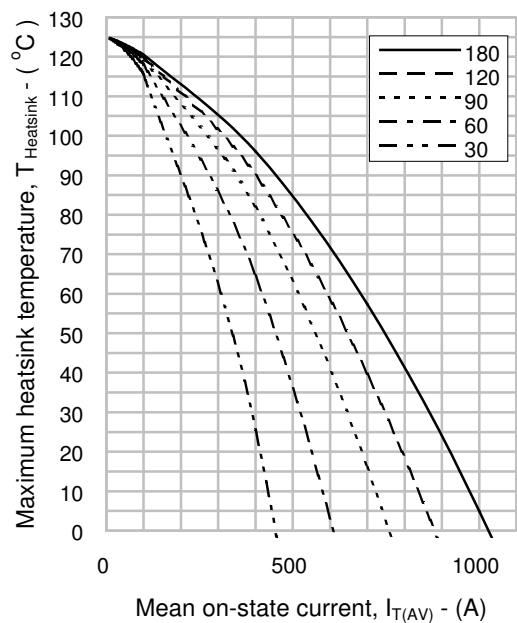
Fig.5 Maximum permissible heatsink temperature, double side cooled – sine wave
