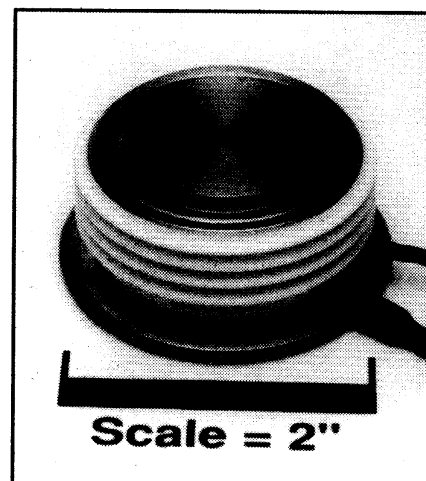
T820 750A Phase Control SCR 750 Amperes Average, 2400 Volts
