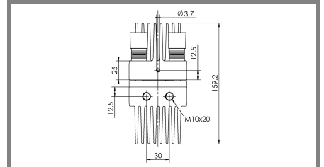
View B
