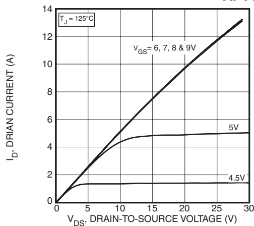
Figure 2, Output Characteristics
