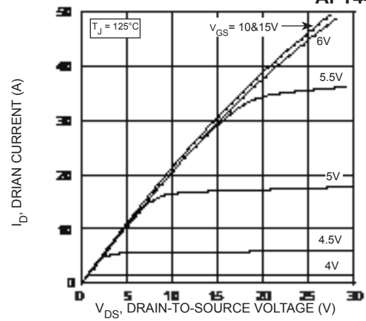
Figure 2, Output Characteristics
