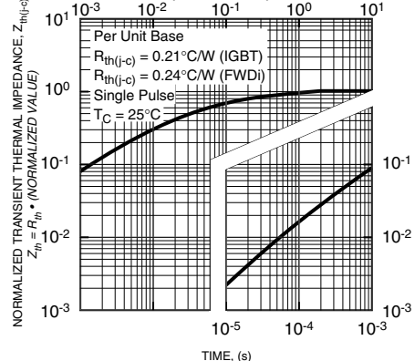
TRANSIENT THERMAL IMPEDANCE CHARACTERISTICS (IGBT & FWDI)
