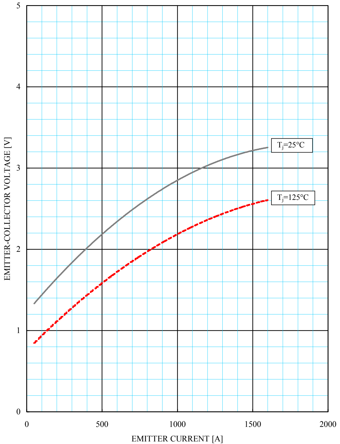
Free wheel diode forward voltage characteristics (typical)
