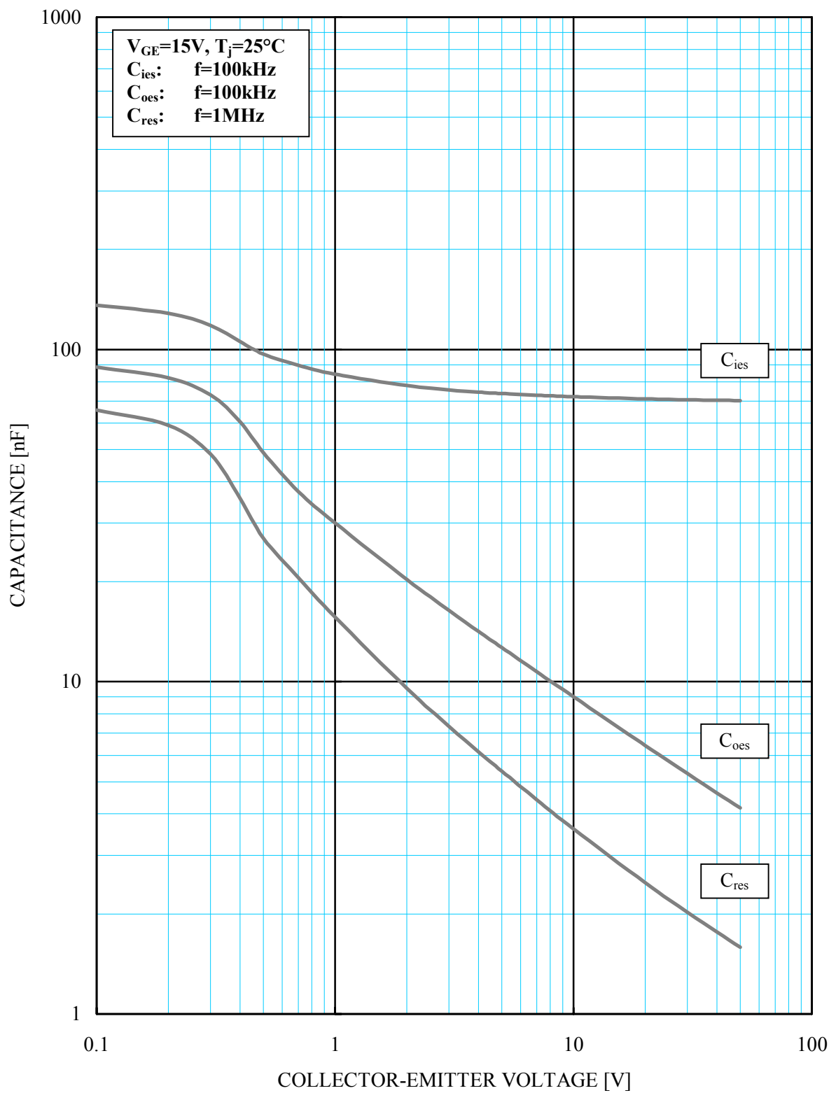
Capacitance characteristics (typical)
