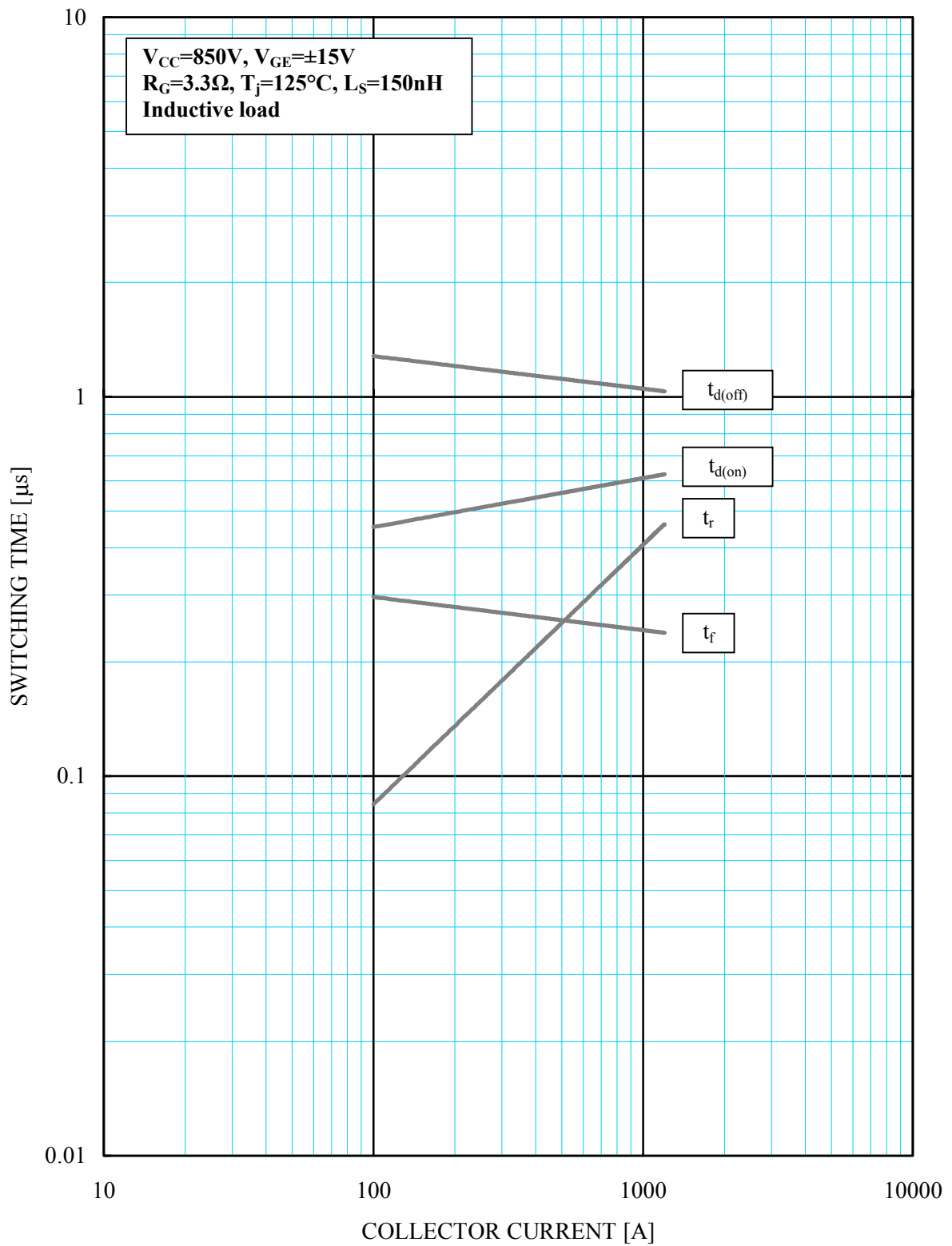
Half-bridge switching time characteristics (typical)
