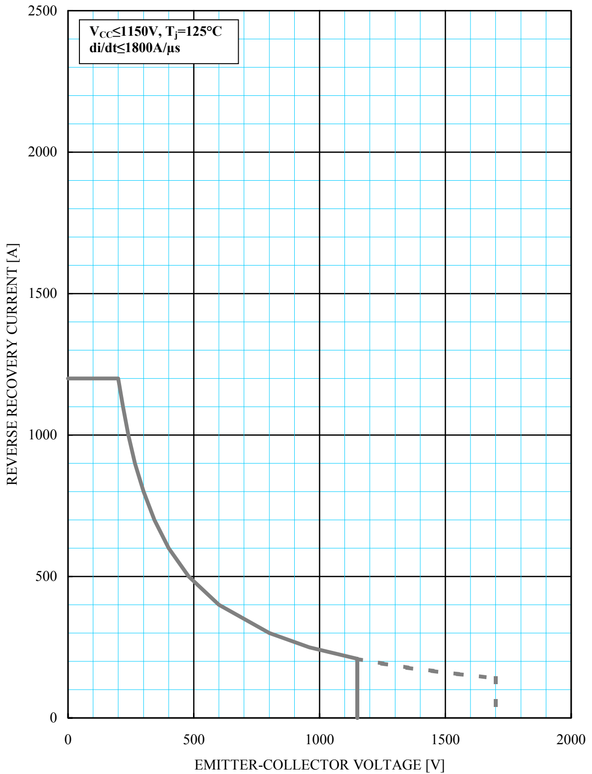
Reverse recovery safe operating area (RRSOA / Di-SOA)
