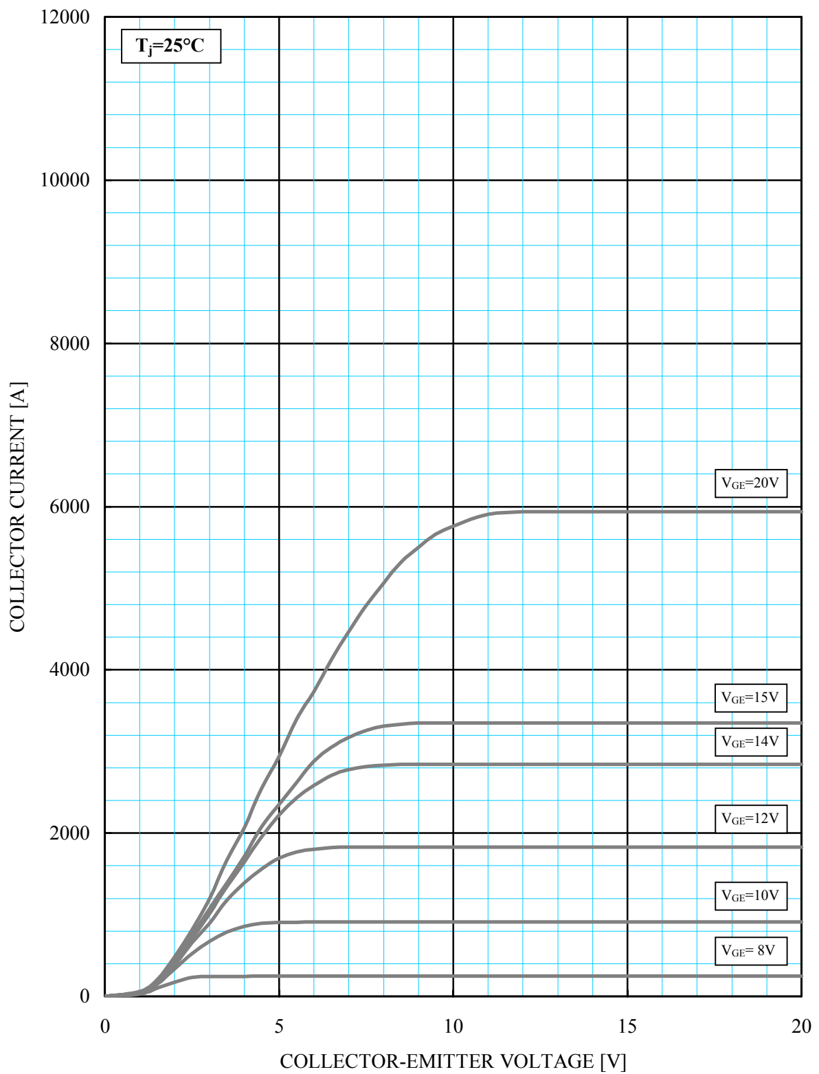
Output characteristics (typical)
