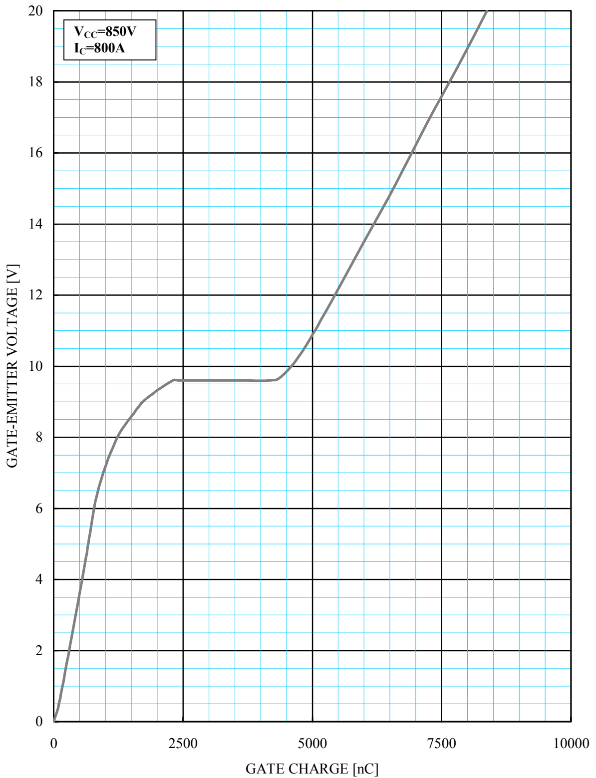
Gate charge characteristics (typical)
