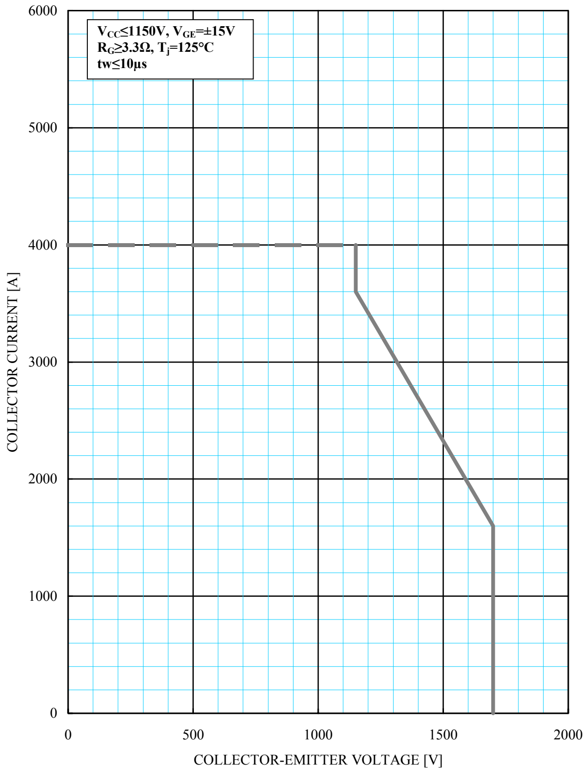
Short circuit safe operating area (SCSOA)
