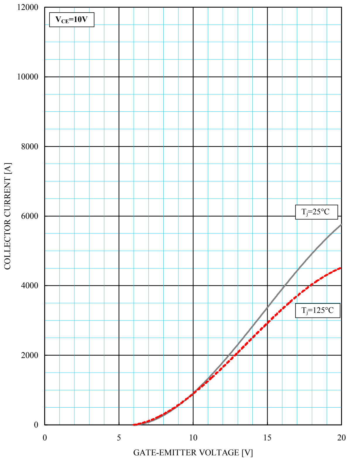
Transfer characteristics (typical)
