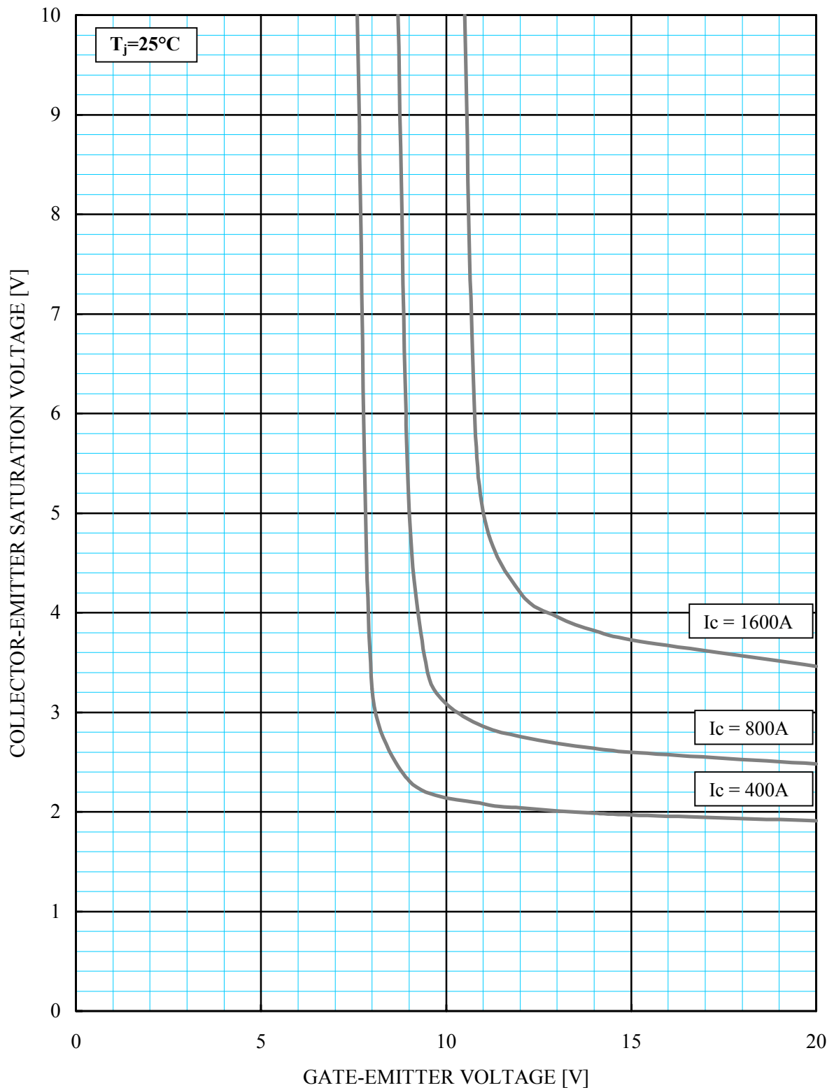
Collector-emitter saturation voltage characteristics (typical)
