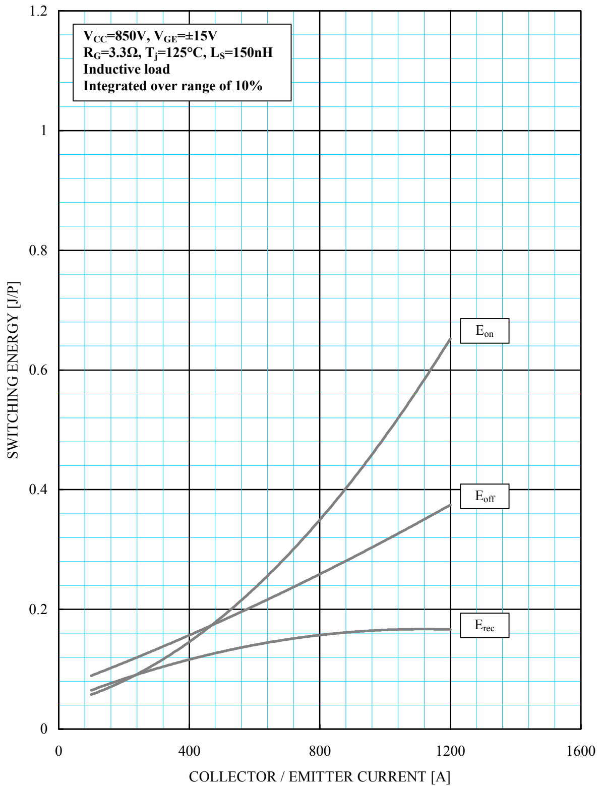
Half-bridge switching energy characteristics (typical)
