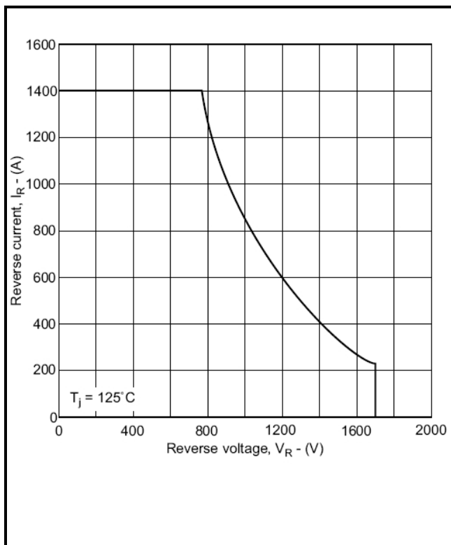
Fig.9 Diode reverse bias safe operating area
