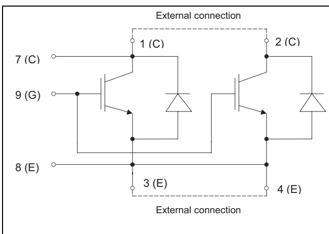
Fig. 1 Circuit configuration
