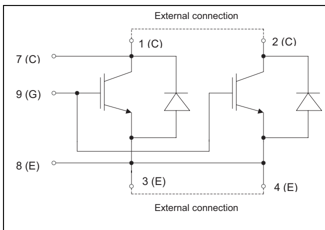
Fig. 1 Circuit configuration
