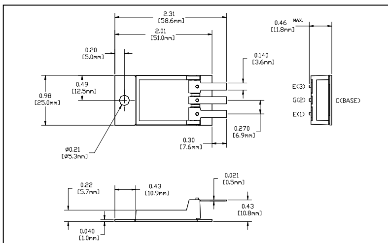
Outline Drawing
