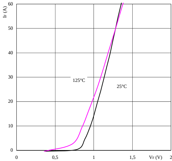
Figure 19. Typical diode forward current as a function of forward voltage
