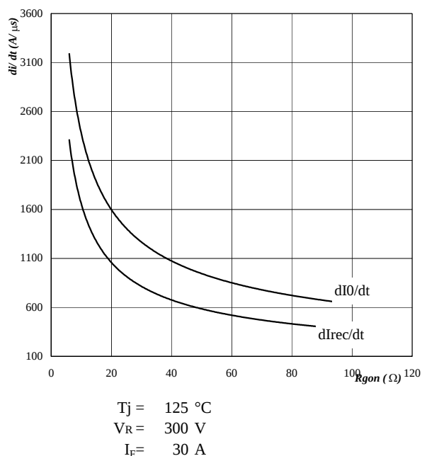
Figure 12. Typical diode peak rate of fall of forward and reverse recovery current as a function of gate resistor Output inverter FRED diode di_0/dt, dI_{rec}/dt = f(R_{gon})
