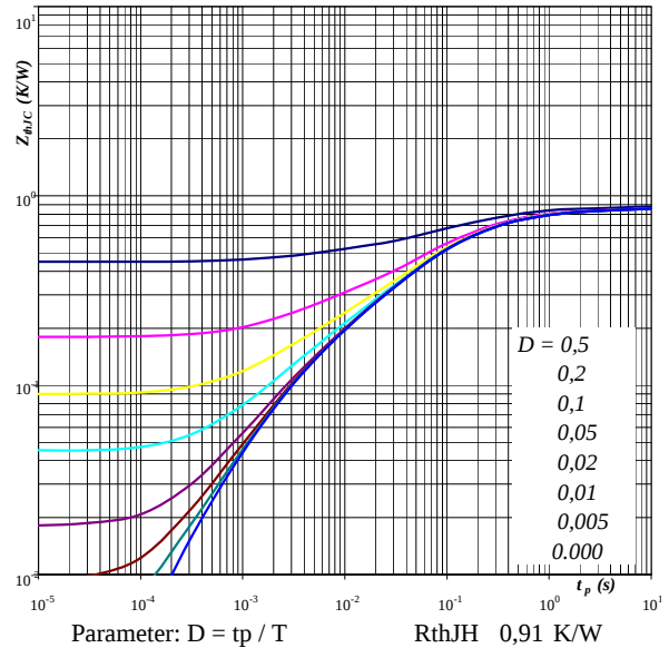
Figure 20. Diode transient thermal impedance as a function of pulse width
