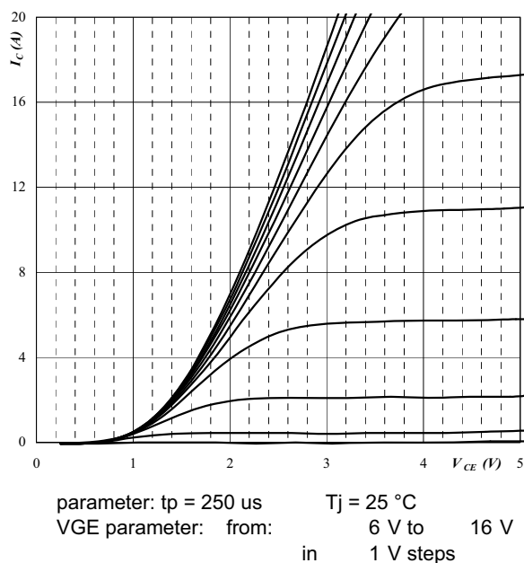
Figure 19. Typical output characteristics Brake IGBT I_c = f(V_{CE})
