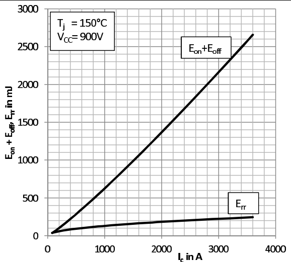
Fig. 4: Typical switching energy E = f(I_C)
