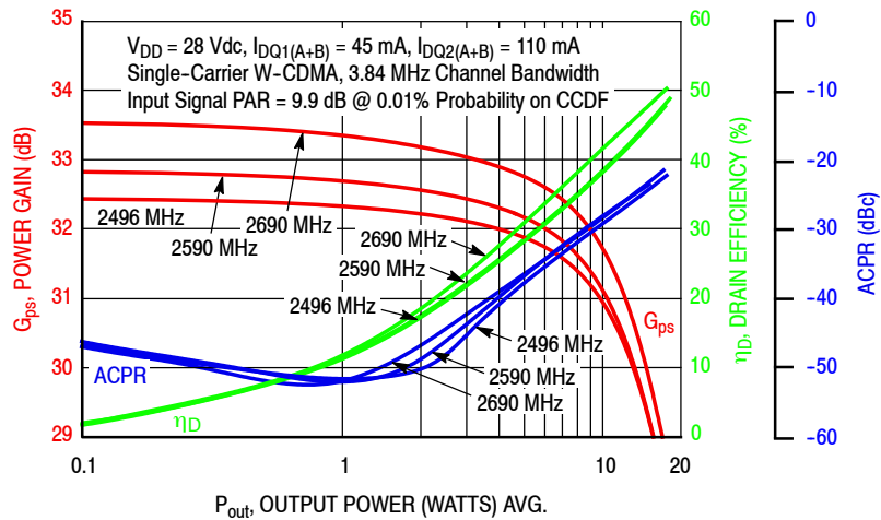
Figure 7. Single-Carrier W-CDMA Power Gain, Drain Efficiency and ACPR versus Output Power — 2496–2690 MHz
