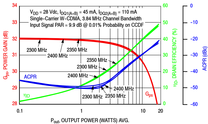
Figure 8. Single-Carrier W-CDMA Power Gain, Drain Efficiency and ACPR versus Output Power — 2300–2400 MHz
