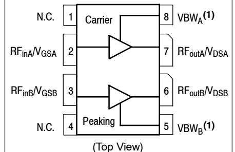
Figure 1. Pin Connections
