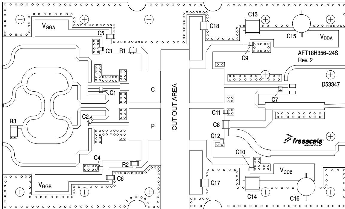
Figure 25. AFT18H356-24SR6 Test Circuit Component Layout — 1930–1995 MHz
