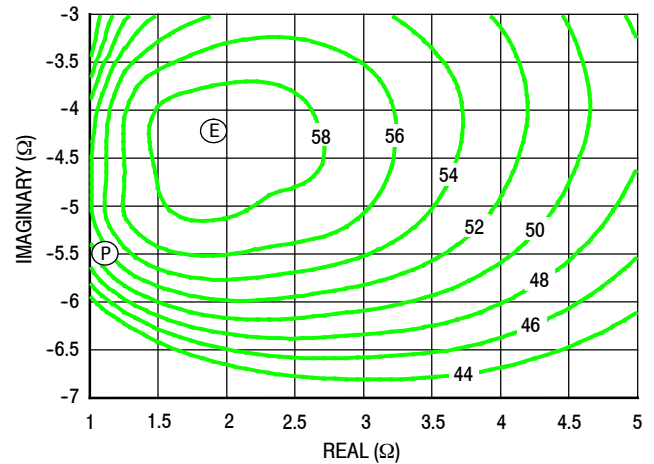
Figure 34. P3dB Load Pull Efficiency Contours (%)
