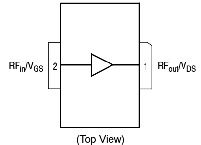
Figure 1. Pin Connections
