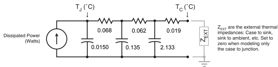
Figure 6b, TRANSIENT THERMAL IMPEDANCE MODEL
