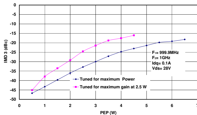
Figure 4 IMD 3 vs. PEP
