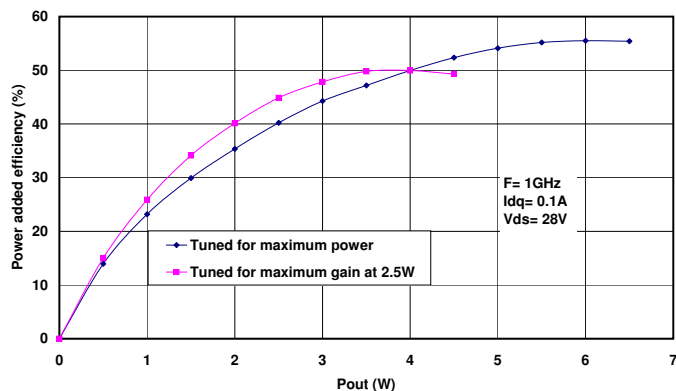
Figure 2 Power added efficiency vs. Output Power.
