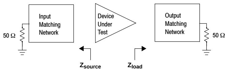
Figure 21. UHF Broadband Series Equivalent Source and Load Impedance — 450–520 MHz
