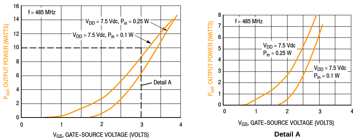
Figure 19. Output Power versus Gate-Source Voltage
