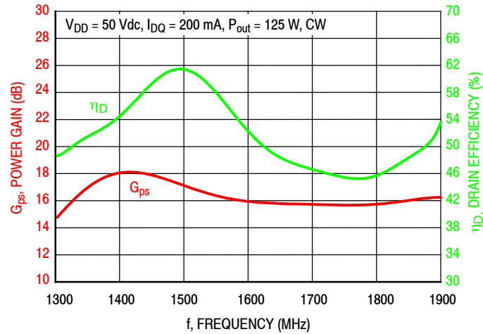
Figure 13. Power Gain and Drain Efficiency versus Frequency
