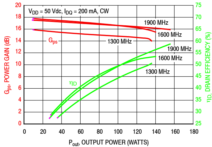
Figure 14. Power Gain and Drain Efficiency versus CW Output Power
