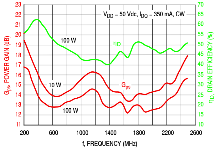
Figure 9. 200–2500 MHz Wideband Circuit Performance
