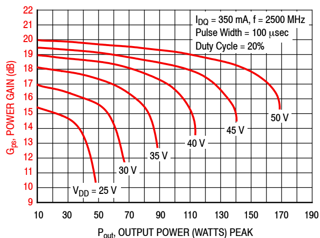
Figure 4. Power Gain versus Output Power (1)
