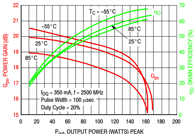
Figure 7. Power Gain and Drain Efficiency versus Output Power (1)
