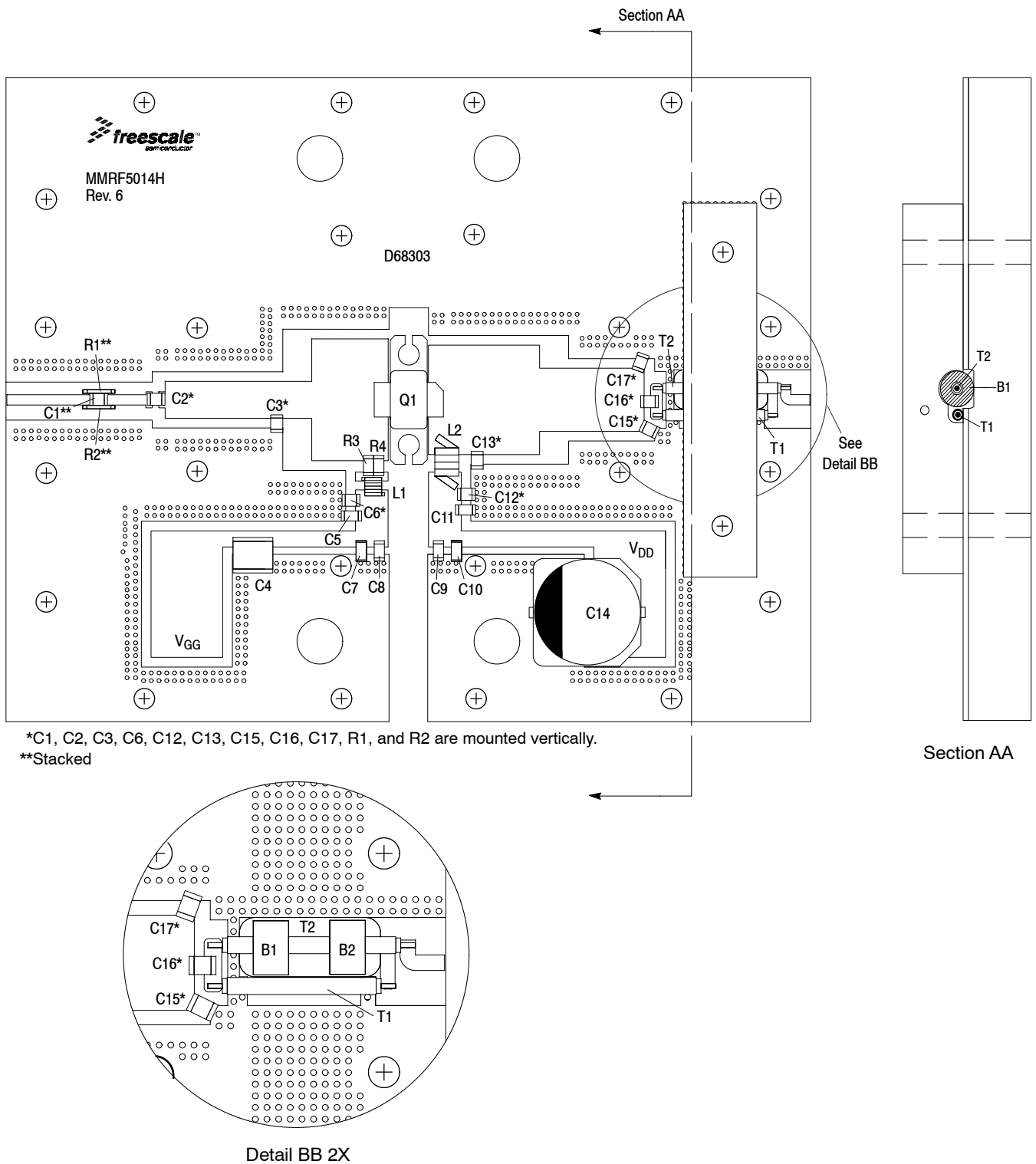
Figure 8. MMRF5014H Wideband Reference Circuit Component Layout — 200–2500 MHz
