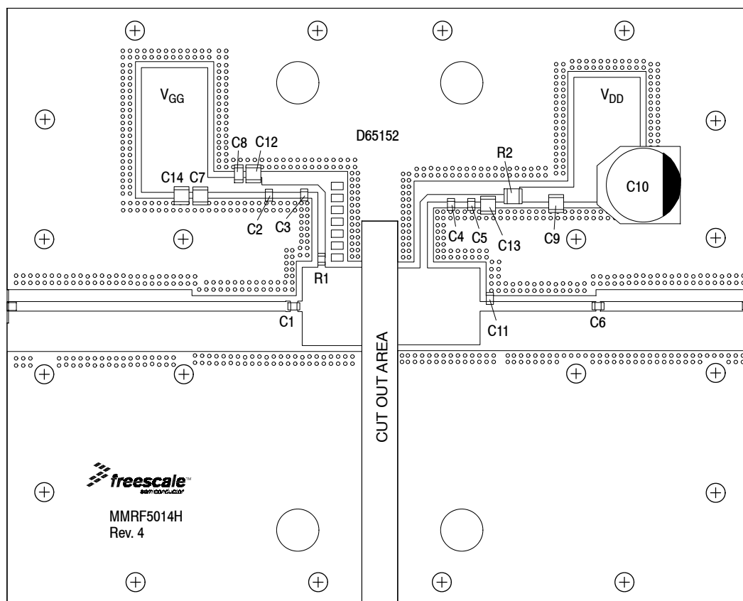
Figure 2. MMRF5014H Narrowband Test Circuit Component Layout — 2500 MHz
