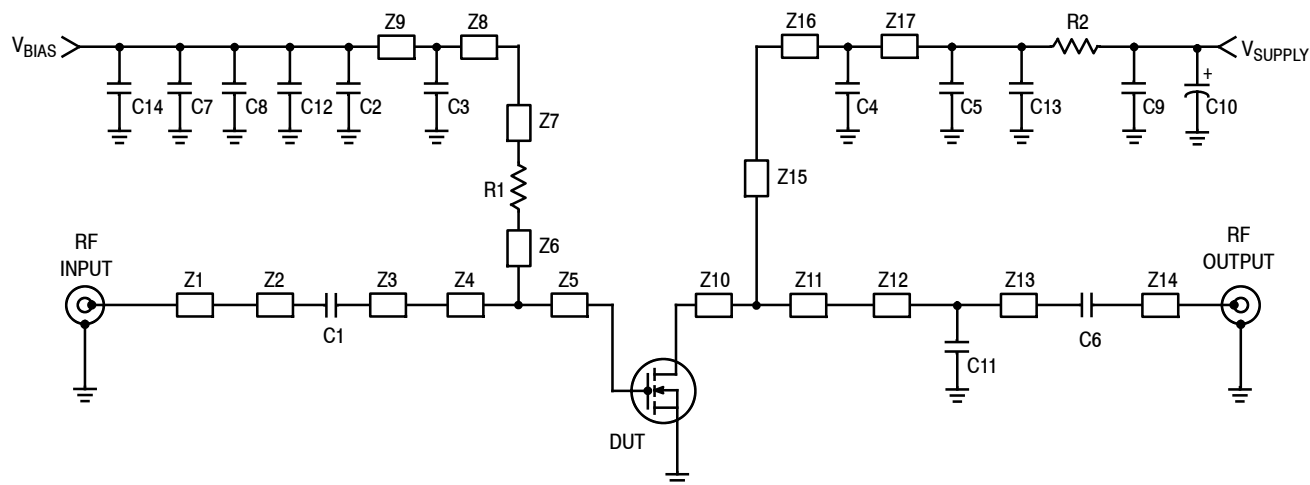
Figure 3. MMRF5014H Narrowband Test Circuit Schematic — 2500 MHz
