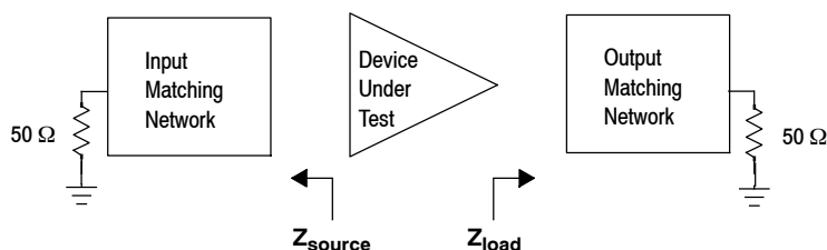
Figure 11. Narrowband Fixtures: Series Equivalent Source and Load Impedances
