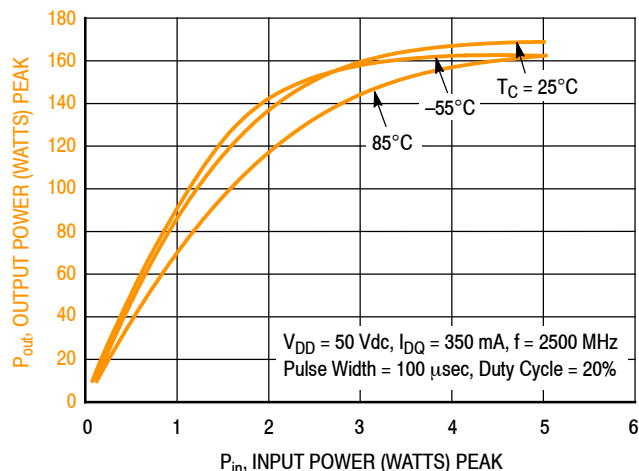
Figure 6. Output Power versus Input Power (1)
