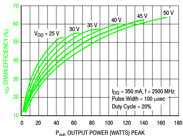
Figure 5. Drain Efficiency versus Output Power (1)
