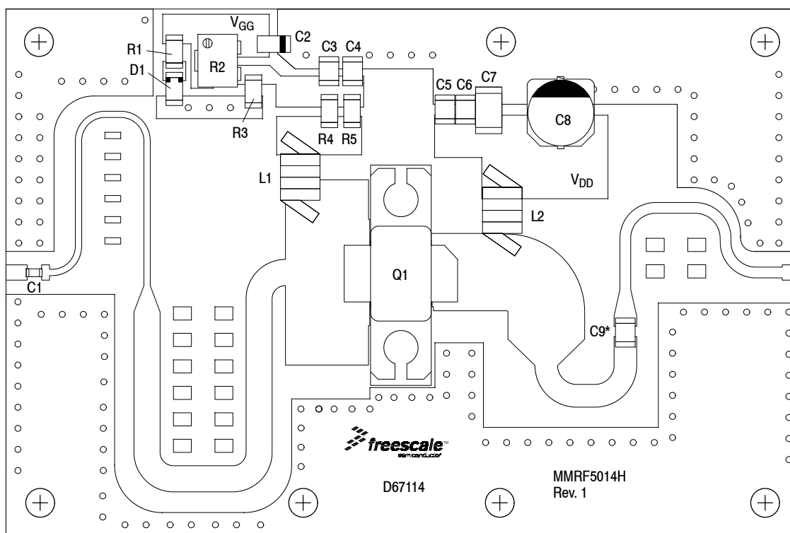
Figure 12. MMRF5014H Wideband Reference Circuit Component Layout — 1300–1900 MHz
