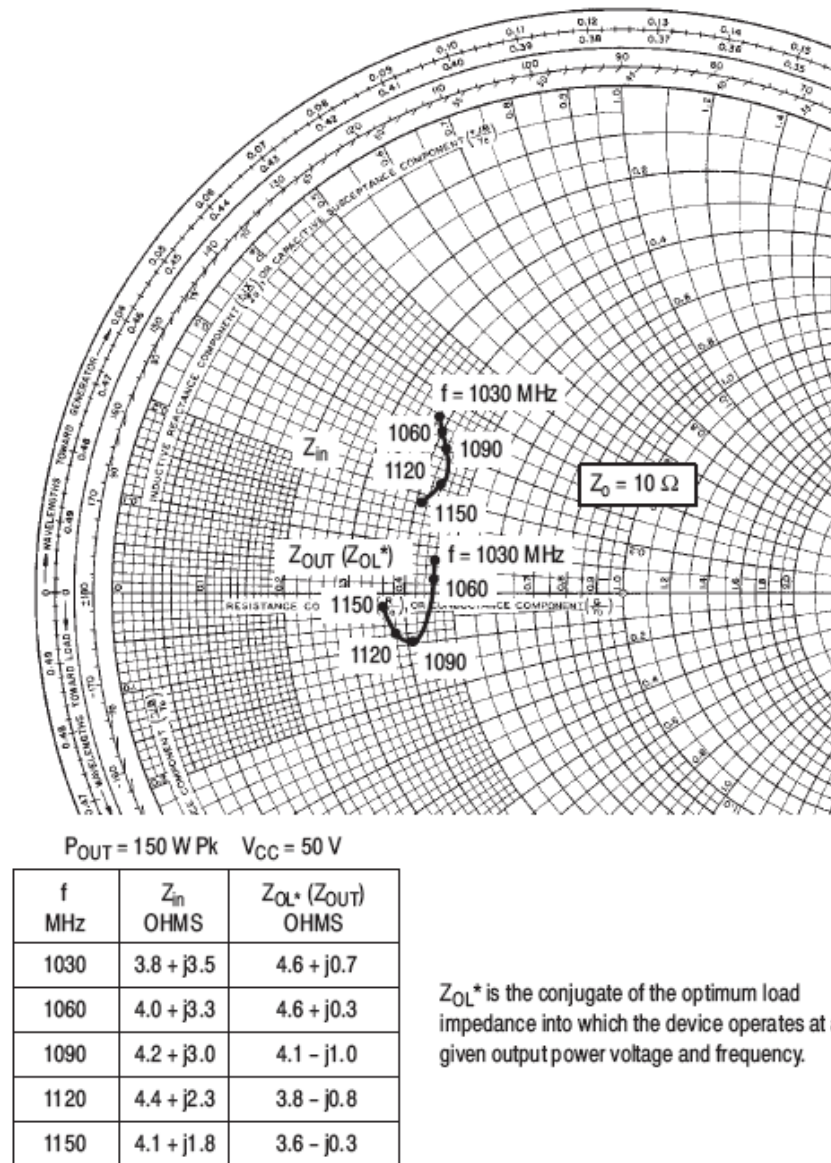
Figure 3. Series Equivalent Input/Output Impedances
