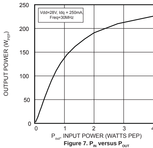
Figure 7. P_{IN} versus P_{OUT}
