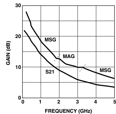
Figure 22. AT-30533 Gains vs. Frequency at V_{CE} = 2.7\text{ V} , I_C = 5\text{ mA} .
