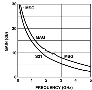
Figure 22. AT-32033 Gains vs. Frequency at V_{CE} = 2.7\text{ V} , I_C = 20\text{ mA} .
