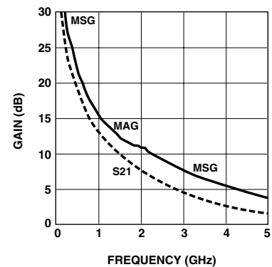
Figure 21. AT-41533 Gains vs. Frequency at V_{CE} = 8V , I_C = 25 \text{ mA} .
