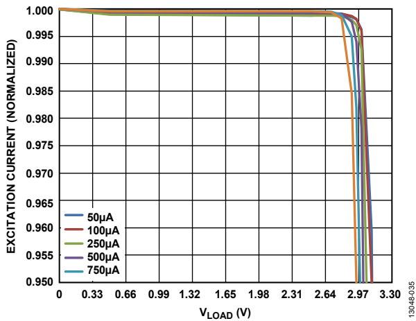
Figure 35. Output Compliance ( AV_{DD} = 3.3V )
