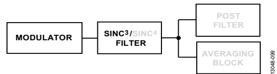
Figure 89. Sinc 3 Filter
