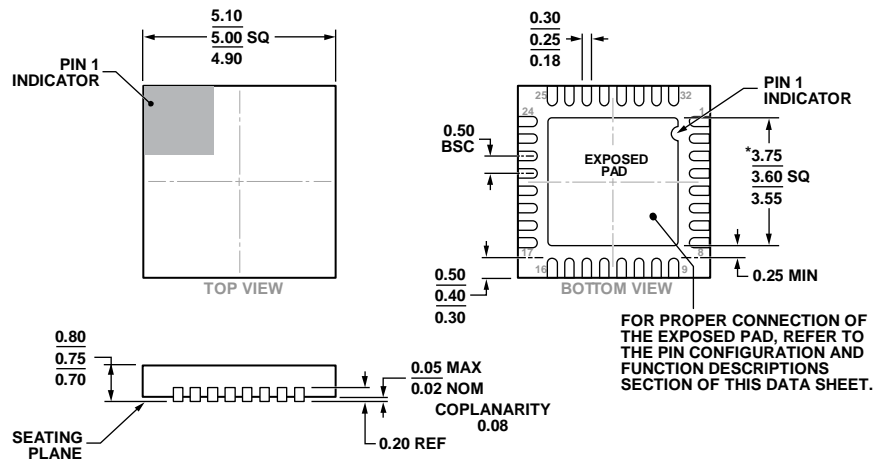
*COMPLIANT TO JEDEC STANDARDS MO-220-WHHD-5 WITH THE EXCEPTION OF THE EXPOSED PAD DIMENSION. Figure 129. 32-Lead Lead Frame Chip Scale Package [LFCSP_WQ] 5 mm x 5 mm Body, Very, Very Thin Quad (CP-32-12) Dimensions shown in millimeters
