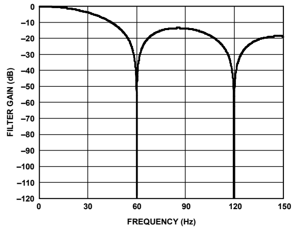
Figure 107. 60 Hz Rejection
