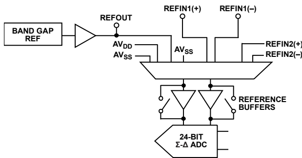
Figure 75. Reference Connections
