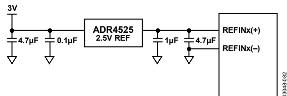
Figure 76. ADR4525 to AD7124-8 Connections
