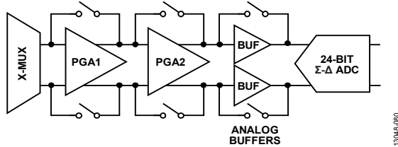
Figure 74. PGA
