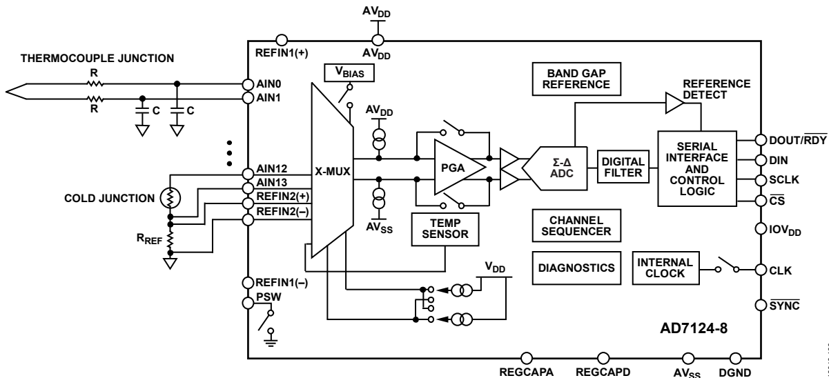
Figure 126. Thermocouple Application
