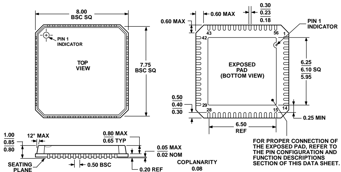
Figure 63. 56-Lead Lead Frame Chip Scale Package [LFCSP_VQ] 8 mm × 8 mm body, Very Thin Quad (CP-56-1) Dimensions shown in millimeters
