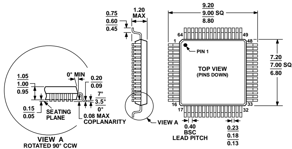
Figure 62. 64-Lead Thin Plastic Quad Flat Package [TQFP] (SU-64-1) Dimensions shown in millimeters
