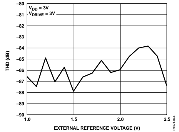
Figure 14. THD vs. Reference Voltage
