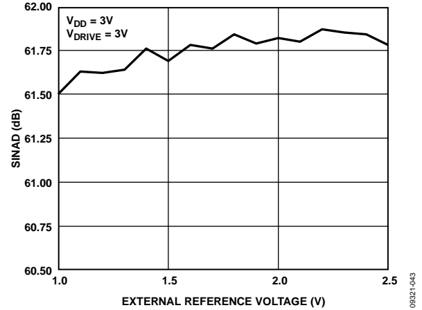
Figure 13. SINAD vs. Reference Voltage
