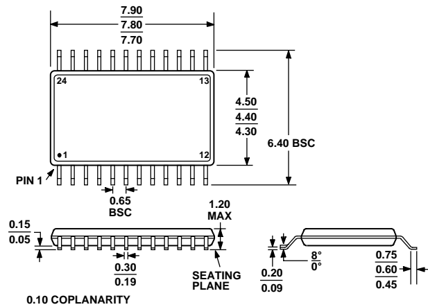
Figure 61. 24-Lead Thin Shrink Small Outline Package [TSSOP] (RU-24) Dimensions shown in millimeters
