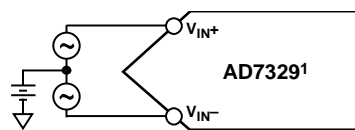
Figure 37. True Differential Inputs
