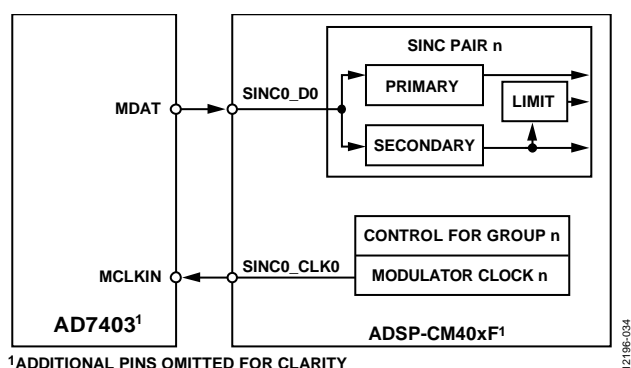
Figure 34. Interfacing the AD7403 to the ADSP-CM40xF
