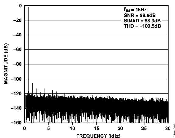
Figure 8. Typical Fast Fourier Transform (FFT)
