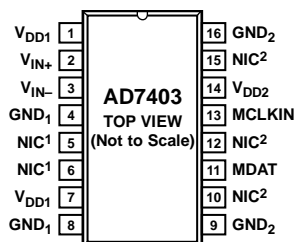
Figure 4. Pin Configuration
