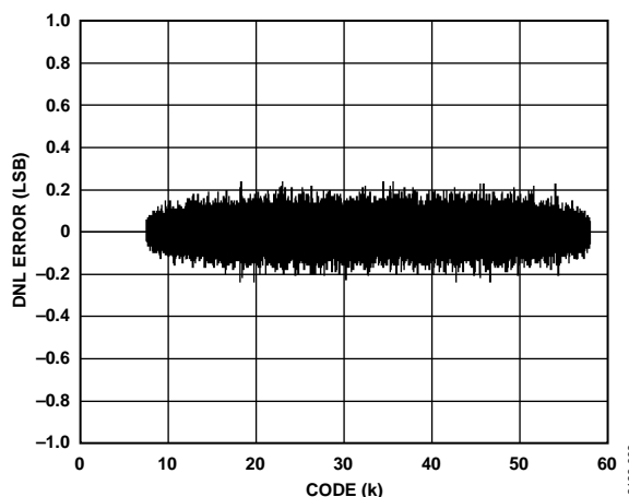
Figure 9. Typical DNL Error
