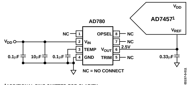
Figure 22. Typical V_{\text{REF}} Connection Diagram for V_{\text{DD}} = 5 V
