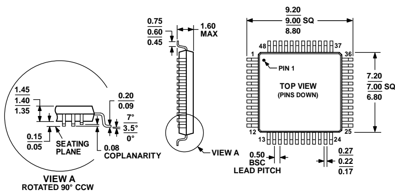
Figure 1. 48-Lead Low Profile Quad Flatpack [LQFP]
