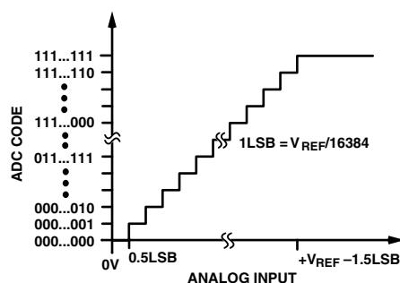
Figure 6. Transfer Characteristic
