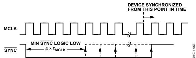
Figure 46. Recommended SYNC Timing
