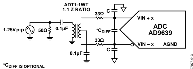
Figure 38. Differential Transformer-Coupled Configuration for Baseband Applications
