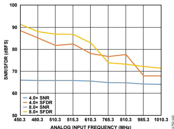
Figure 67. SNR/SFDR vs. f_{IN} ; 500 MHz < f_{IN} < 1 GHz; Buffer Control 1 (0x018) = 4.0\times and 8.0\times
