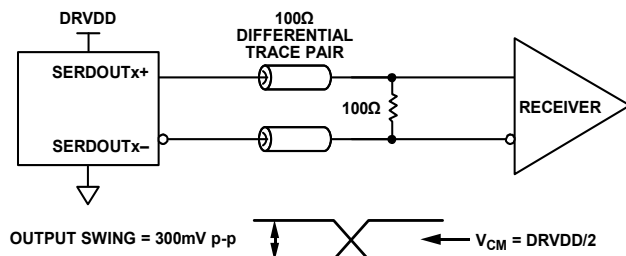
Figure 133. DC-Coupled Digital Output Termination Example
