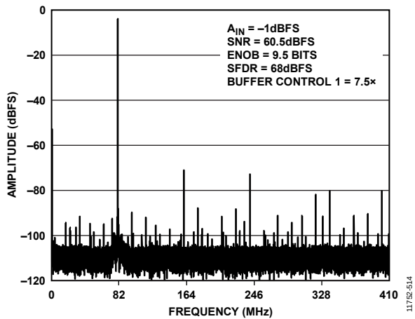
Figure 38. Single-Tone FFT with f_{IN} = 1720.3 MHz
