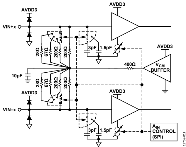
Figure 80. Analog Inputs
