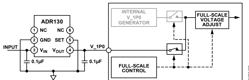
Figure 106. External Reference Using ADR130
