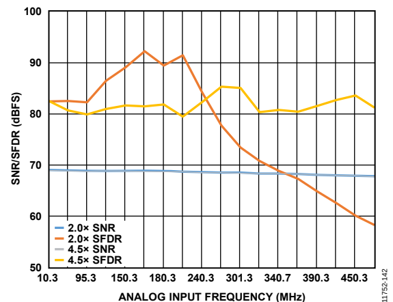
Figure 66. SNR/SFDR vs. f_{IN} ; f_{IN} < 500 MHz; Buffer Control 1 (0x018) = 2.0\times and 4.5\times
