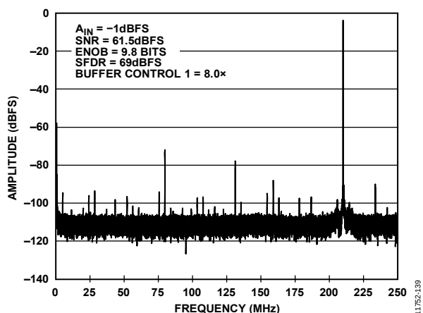
Figure 63. Single-Tone FFT with f_{IN} = 1710.3 MHz
