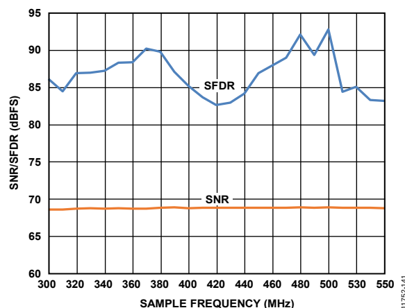
Figure 65. SNR/SFDR vs. f_s , f_{IN} = 170.3 MHz; Buffer Control 1 = 2.0\times
