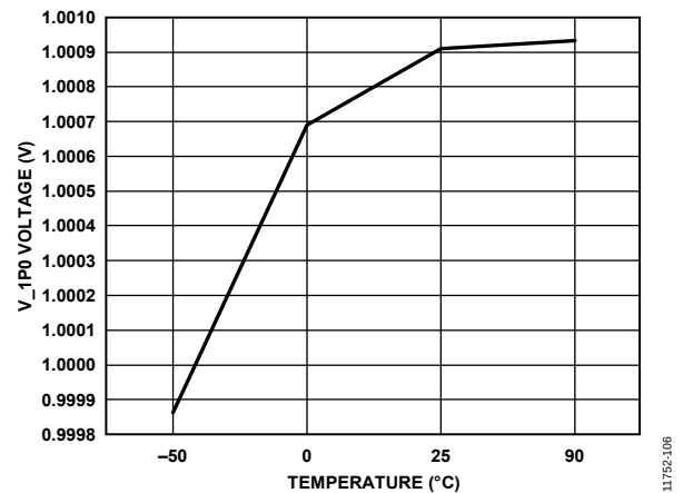
Figure 105. Typical V_1P0 Drift
