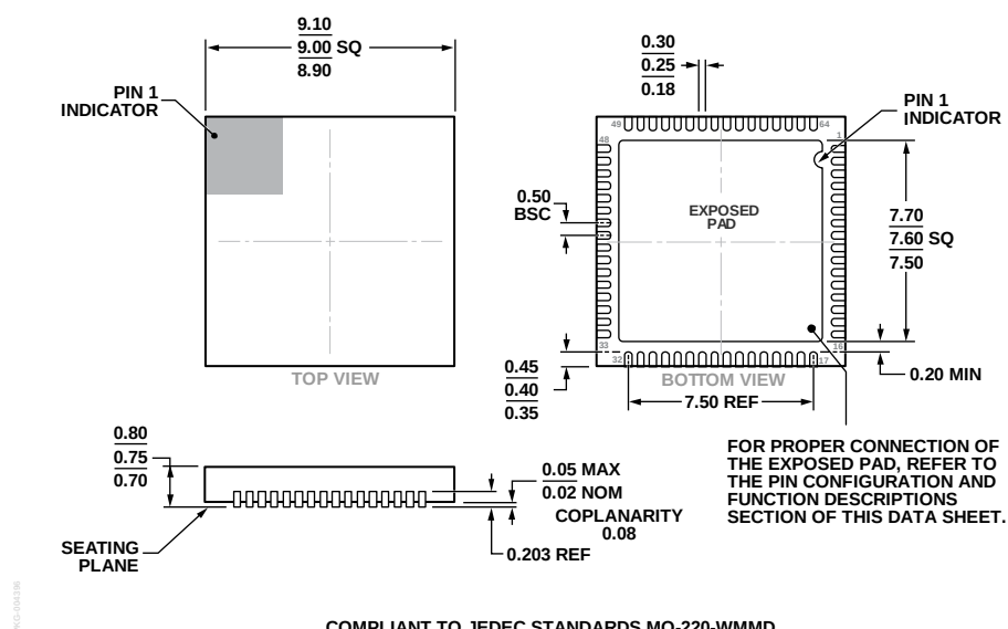
Figure 149. 64-Lead Lead Frame Chip Scale Package [LFCSP_WQ] 9 mm × 9 mm Body, Very Thin Quad (CP-64-15) Dimensions shown in millimeters
