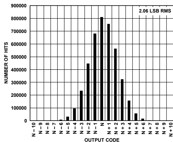
Figure 77. Input-Referred Noise Histogram
