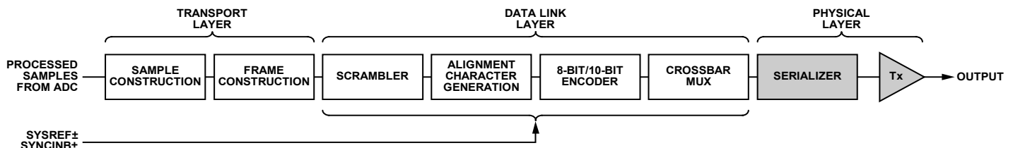
Figure 130. Data Flow
