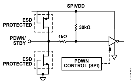
Figure 89. PDWN/STBY Input
