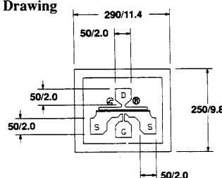
CF004 CHIP (UNITS IN MICRONS/MILS) THICKNESS: 110 MICRONS/4.3 MILS
