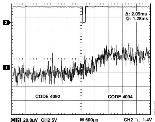
Figure 35. DAC Output with 300 Hz Filter on Output
