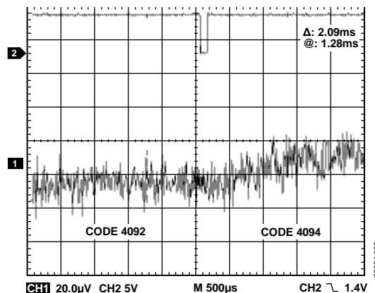
Figure 34. DAC Output with 50 Hz Filter on Output
