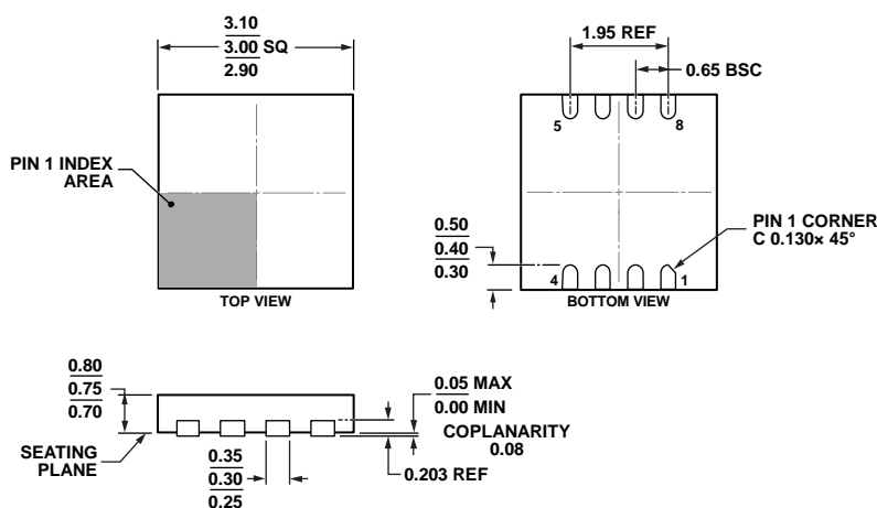
Figure 39. 8-Lead Lead Frame Chip Scale Package [LFCSP_WD] 3 mm × 3 mm Body, Very Very Thin, Dual Lead (CP-8-15)
