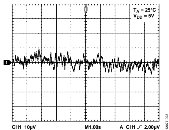
Figure 27. Internal Reference Noise, 0.1 Hz to 10 Hz
