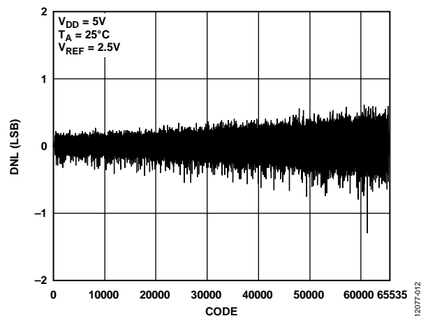
Figure 11. AD5693R DNL
