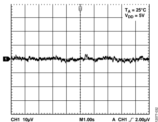
Figure 31. 0.1 Hz to 10 Hz Output Noise Plot, External Reference
