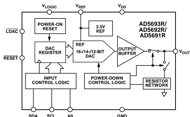
Figure 1. MSOP
