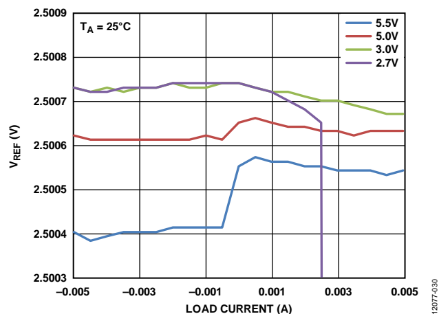
Figure 29. Internal Reference Voltage vs. Load Current
