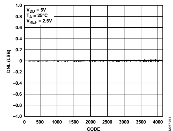
Figure 13. AD5691R DNL
