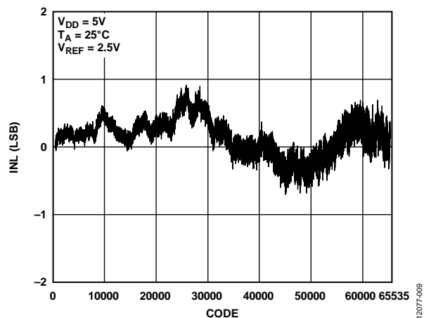
Figure 8. AD5693R INL
