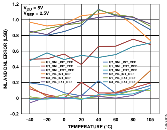
Figure 14. INL and DNL Error vs. Temperature (AD5693R)
