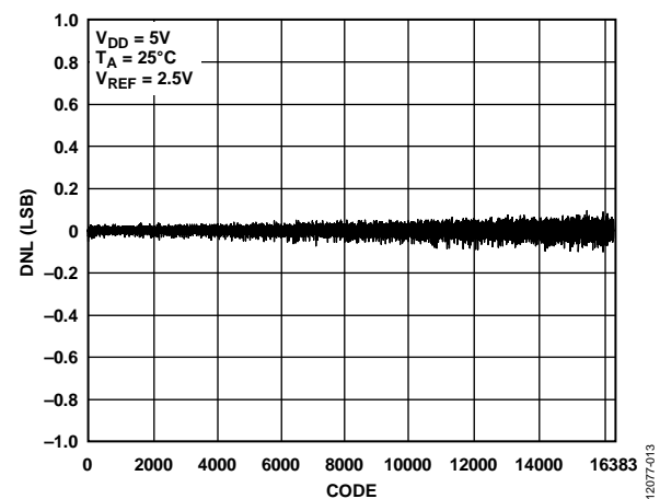
Figure 12. AD5692R DNL
