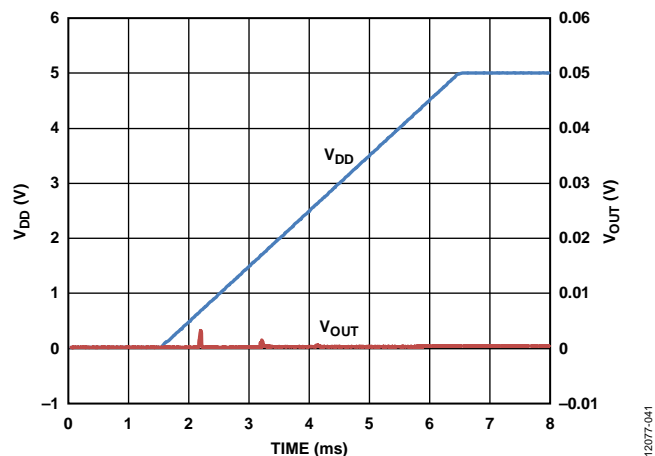
Figure 40. Power-On Reset to 0 V
