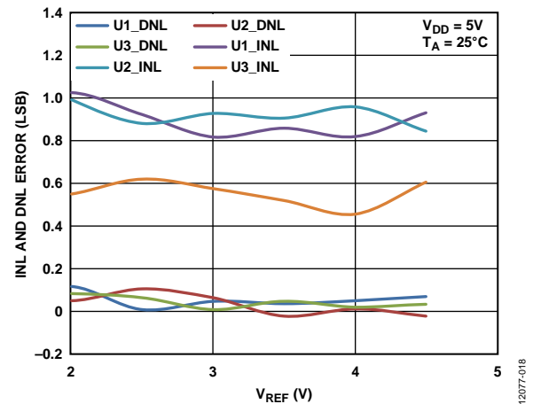
Figure 17. INL and DNL Error vs. V_{REF} (AD5693R)
