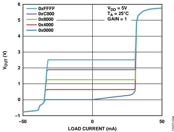
Figure 33. Source and Sink Capability, Gain = 1
