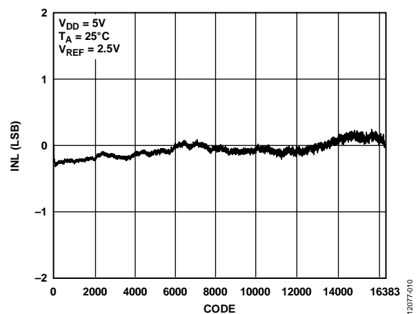
Figure 9. AD5692R INL
