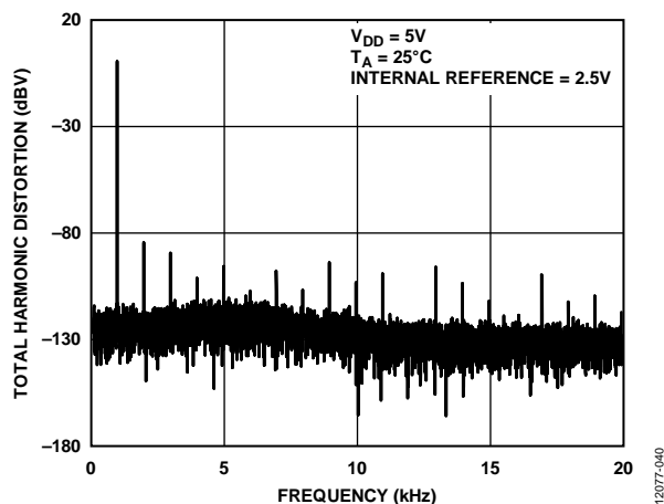
Figure 39. Total Harmonic Distortion at 1 kHz
