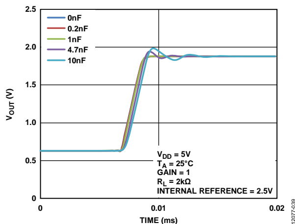
Figure 38. Capacitive Load vs. Settling Time, Gain = 1
