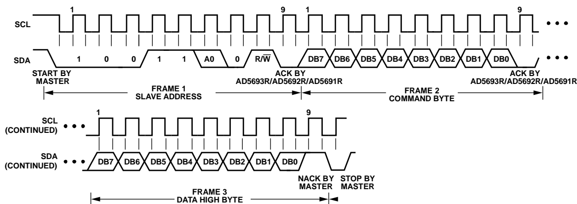
Figure 48. I²C Read Operation
