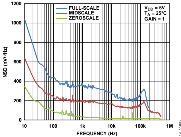
Figure 32. Noise Spectral Density vs. Frequency, Gain = 1
