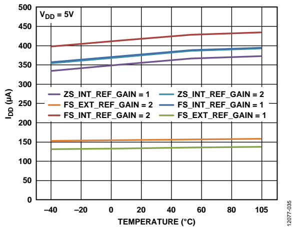
Figure 34. I_{DD} vs. Temperature
