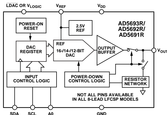
Figure 2. LFCSP
