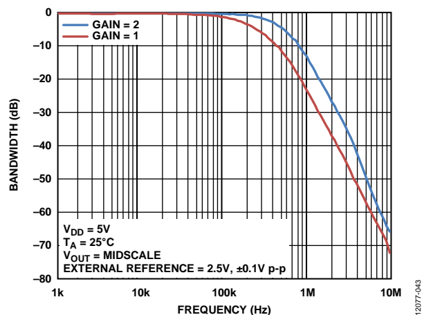
Figure 42. Multiplying Bandwidth, External Reference = 2.5 V, \pm 0.1 V p-p, 10 kHz to 10 MHz
