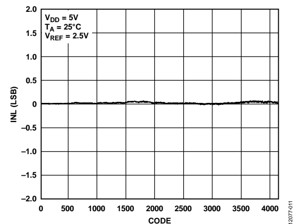
Figure 10. AD5691R INL
